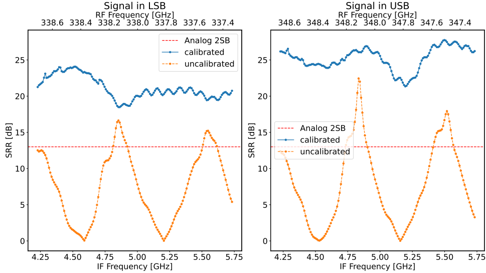
Figure 1: Exemplary SRR, comparing the measured, digitally calibrated (blue) and uncalibrated SRRs (orange) to the specified analog performance (red) of an ALMA Band 7 SIS mixer in a test setup.
