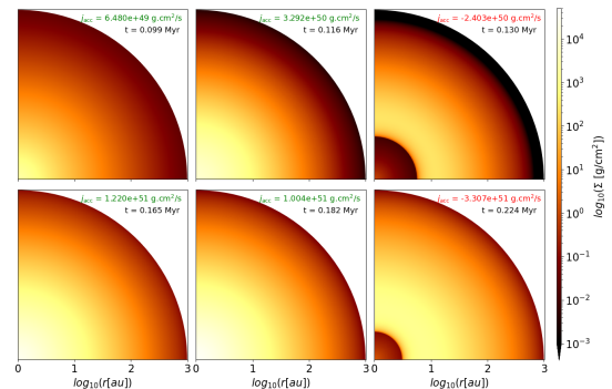
Figure 1: 2D view of the surface density evolution of the second sink particles formed in the fiducial run 1 . j_{\text{acc}} is shown in green (red) when positive (negative) to highlight the correlation between the disk shape and the accreted angular momentum sign.
