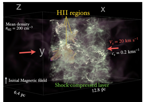
Figure 1: Three-dimensional radiation MHD simulation of a shock-compressed layer formed by supersonic flows in a molecular cloud. Dense filamentary structures and HII regions develop within the compressed layer.
