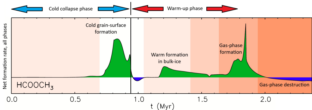
Figure 1: Net formation rate of methyl formate (HCOOCH 3 ) as a function of time, summed over all phases (gas + surface + bulk ice), during a representative hot-core chemical model.
