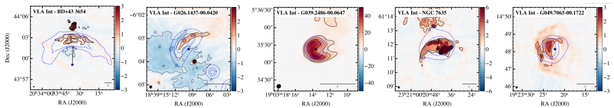
Figure 1: Radio observations of 5 bow-shock nebulae (Moutzouri+ 2025): VLA intensity map in \text{mJy beam}^{-1} with blue contours of WISE mid-IR emission overlaid.
